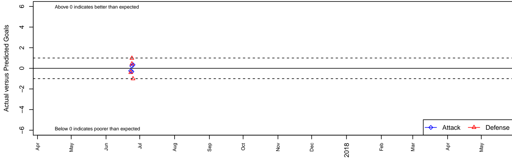
El Dorado Hills SC Fusion G99 Dots are actual minus expected GF (blue circles) and GA (red triangles). Blue line is smoothed change in attack strength. Red is smoothed change in defense strength.
